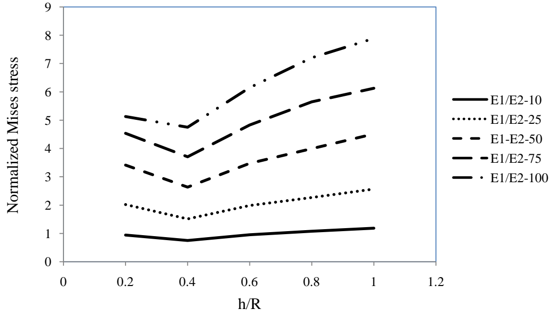
Figure 5.4-7 Variation of Maximum Mises Stress for Hard Thin Film over Soft Substrate Model
